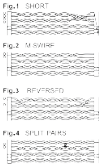
Fault details
